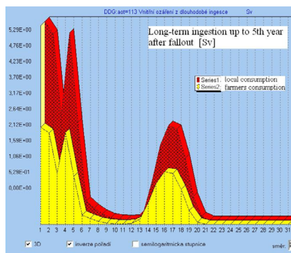
Fig. 8a Committed ingestion dose averted due to food bans in consumption (reduced contaminated consumption basket, polar angle beam 21)
