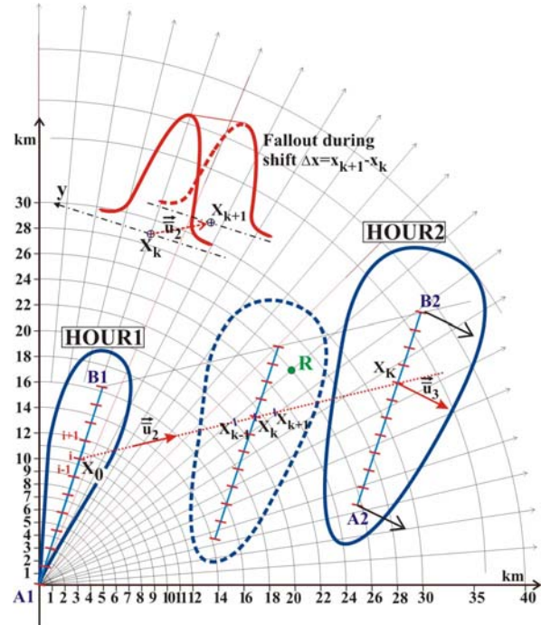
Fig. 1 Segmented Gaussian plume approach for modeling of discharges propagation in atmosphere
