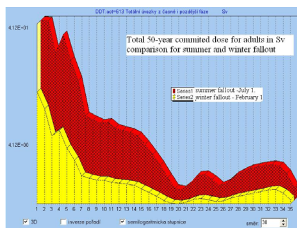
Fig. 8b 50-years total committed dose for adults for summer fallout in July 1 (in red) and winter fallout in February 1 (yellow). Shape in polar angle 30.
