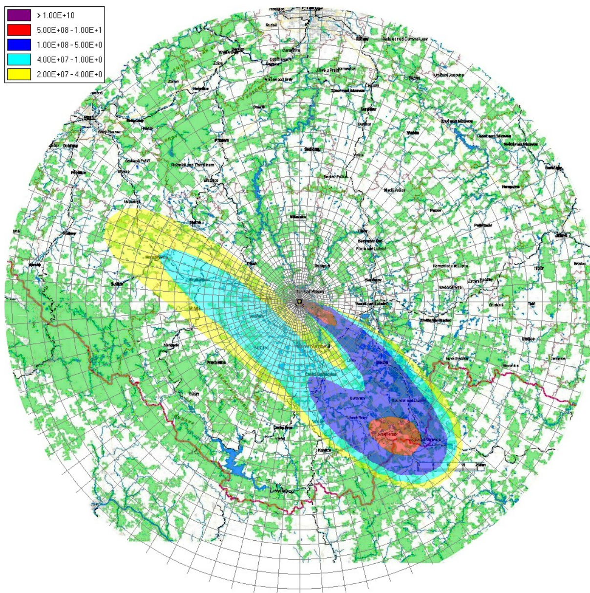
Fig. 4 Deposited activity of I131 after 32 hours after the release start at 12.00 UTM on Feb. 22, 2007. After 8 hours the wind direction changed to nearly opposite orientation (the forecast confirmed by latter measurements)
