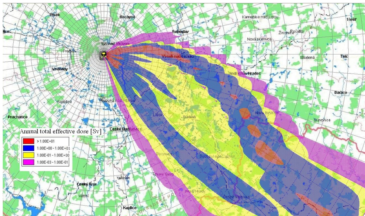
Fig. 5 Total annual effective dose for adults [Sv] in the first year of release. Source term ST2 – severe LOCA accident with fuel melting, meteorological forecast for June 28, 2002, 00 UTM. Conservative “Local production \times Local consumption” ingestion scheme.
