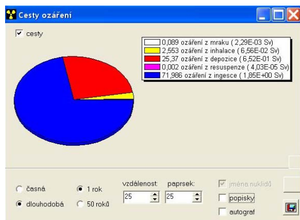
Fig. 6b Percentage contribution of particular irradiation pathway to annual effective dose for adults – scenario MELK-STEP II .
