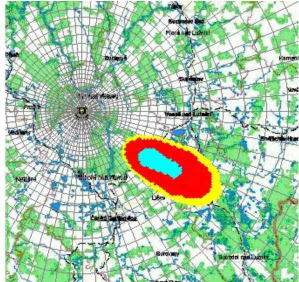
Fig. 3a Near-ground activity concentration of I131 just after 2 nd hour after release start
