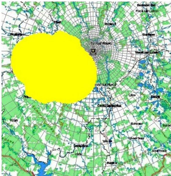
Fig. 3c Near-ground activity concentration of I131 just after 25 th hour after release start (movement in opposite direction back to NPP Temelin)
