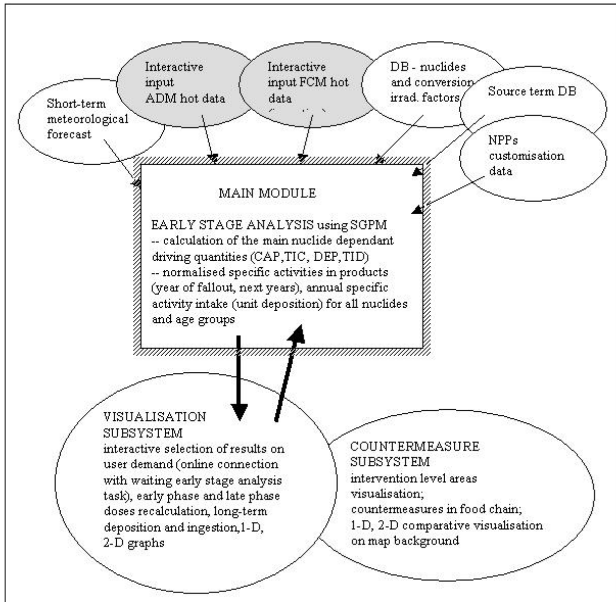
Fig. 2 Diagram of deterministic root of the HARP system
