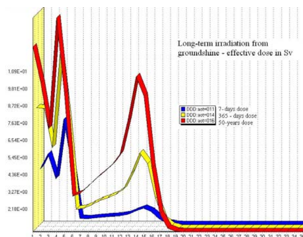
Fig. 7a Groundshine dose – time evolution - angular direction south-east (polar angle beam 20)
