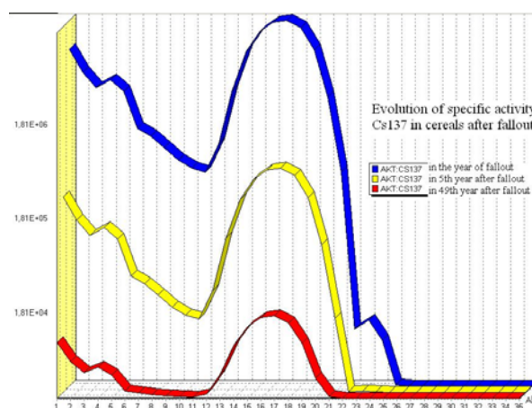
Fig. 7b Time evolution of Cs137 specific activity in cereals [Bq.kg -1 ] (polar angle beam 21)
