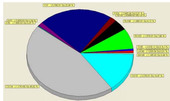
Fig. 6a Percentage nuclide contribution to annual effective dose for adults – scenario MELK-STEP II
