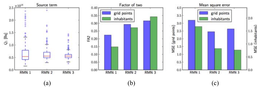
Figure 2 (a) Boxplots for ensembles of estimates of activity release Q_1 for assessed networks (median, box at 25% and 75% quantile, and crosses denote outlying realisations), (b) Values of the FA2 loss function (c) Values of the MSE loss function (see online version for colours)
