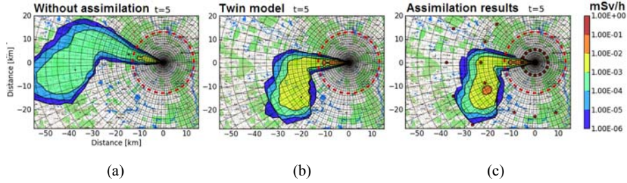
Figure 3 (a) Simple model prediction of dose rate: D^{nom} = M(\theta_{nom}) without accounting of measurements (b) Twin model: D^{win} = M(\theta_{win}) (c) Assimilation scheme: \hat{D} = M(\theta_{asim}(y), \theta_{other}) – assimilation with the true release represented by the twin model (see online version for colours)
